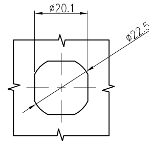
PANEL DRILLING DIMENSIONS
