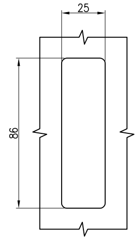
Panel Drilling Dimensions
