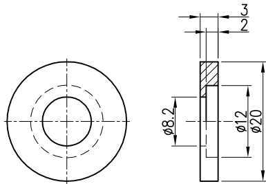
WASHER (SCALE 1:2)
