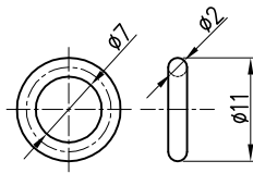
O-RING (SCALE 1:2)
