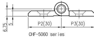
CHF-5060 series
