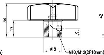
CA-2043L / NUT TYPE
