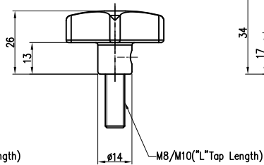
CA-2043M / BOLT TYPE
