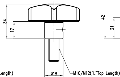
CA-2043L / BOLT TYPE
