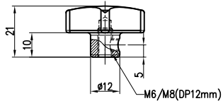
CA-2043S / NUT TYPE
