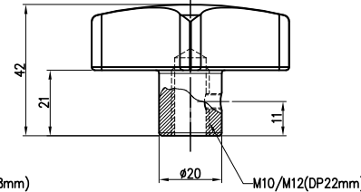
CA-2043XL / NUT TYPE
