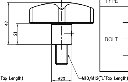
CA-2043XL / BOLT TYPE
