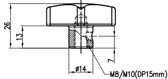
CA-2043M / NUT TYPE
