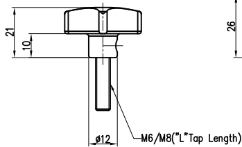
CA-2043S / BOLT TYPE
