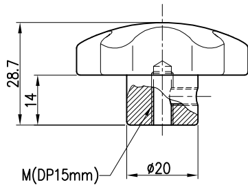
CA-1056L / NUT TYPE
