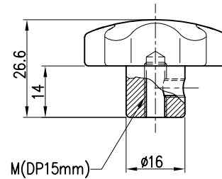
CA-1056M / NUT TYPE
