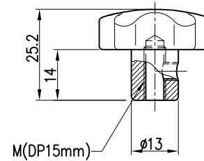
CA-1056S / NUT TYPE
